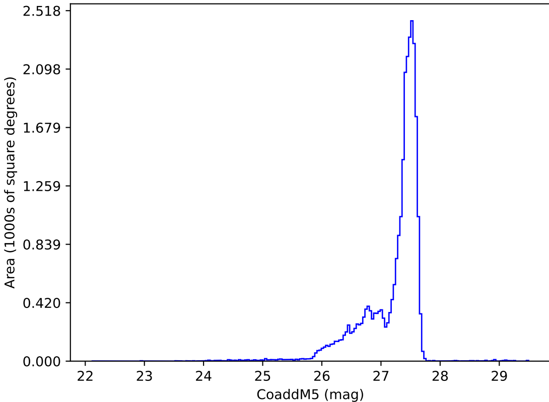
too_elab_r8_d2_giz_v3.4_10yrs : CoaddM5
