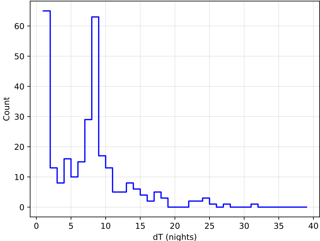
too_elab_r8_d2_giz_v3.4_10yrs all bands: DD:XMM_LSS Delta Nights Histogram
