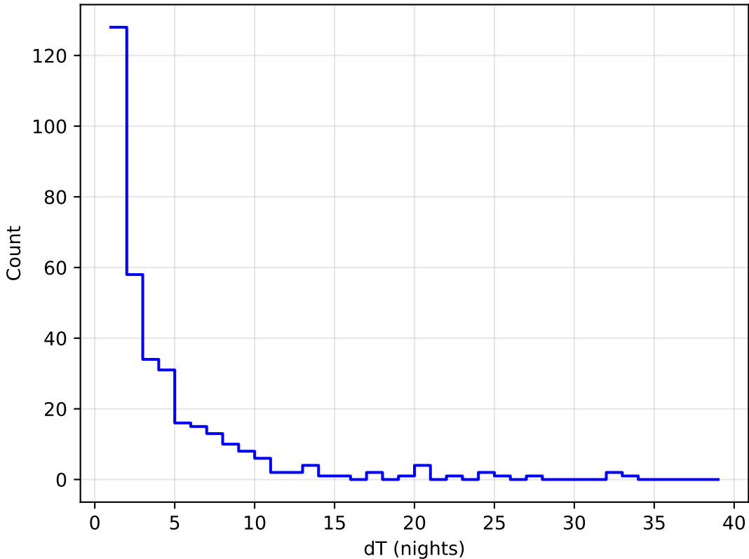
too_elab_r8_d2_giz_v3.4_10yrs all bands: DD:WFD Delta Nights Histogram
