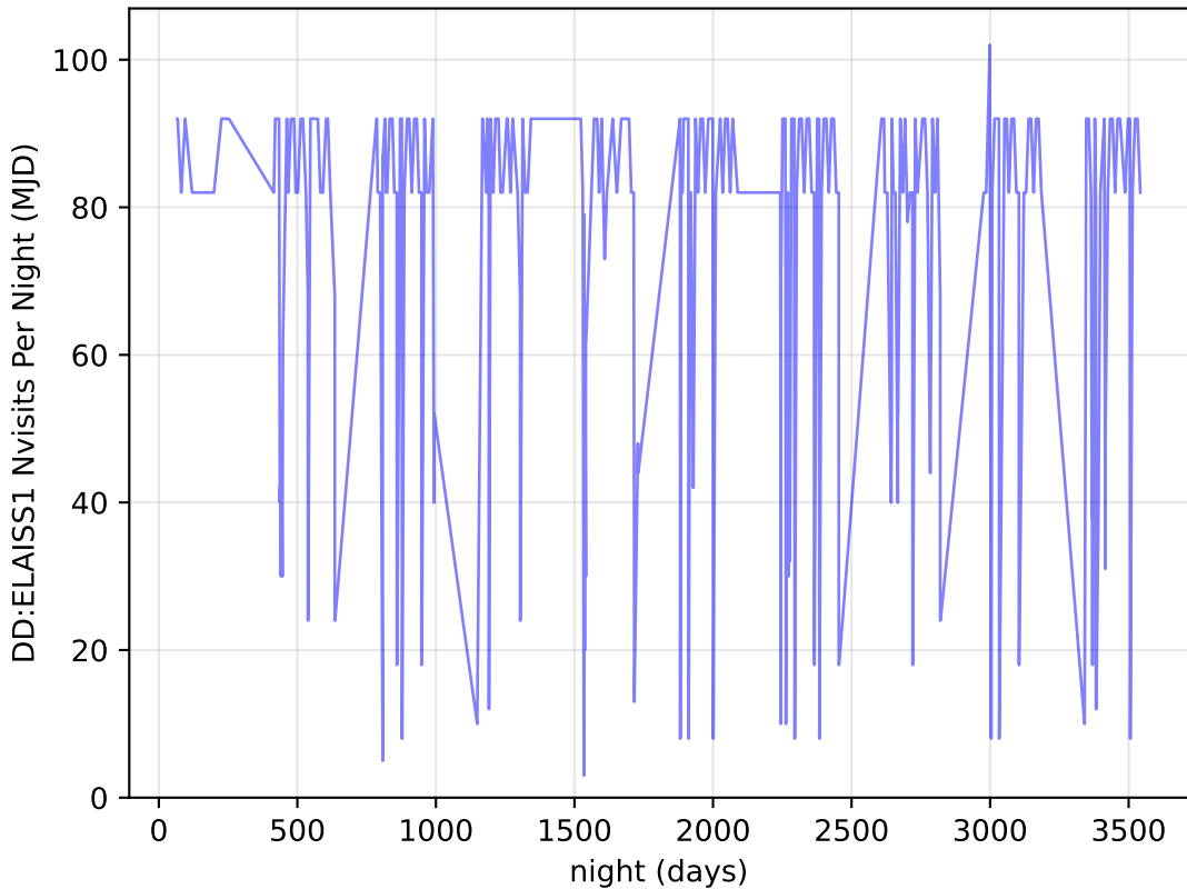
too_elab_r8_d2_giz_v3.4_10yrs all bands: DD:ELAISS1 Nvisits Per Night
