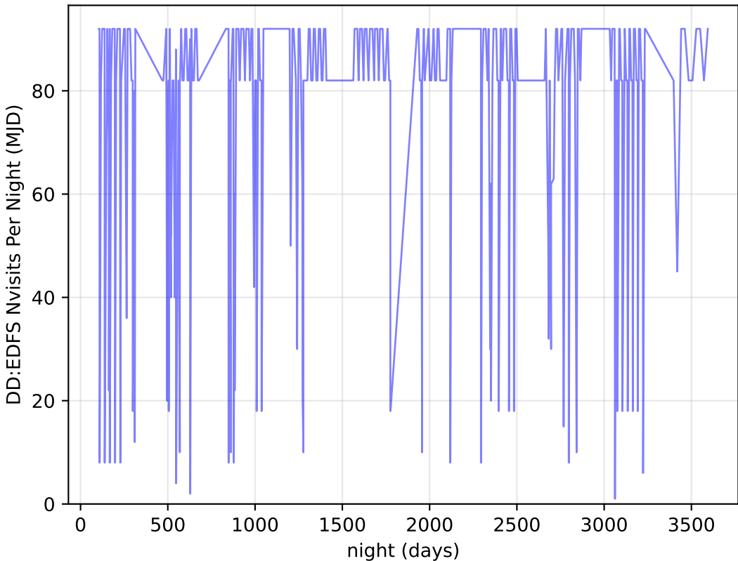
too_elab_r8_d2_giz_v3.4_10yrs all bands: DD:EDFS Nvisits Per Night
