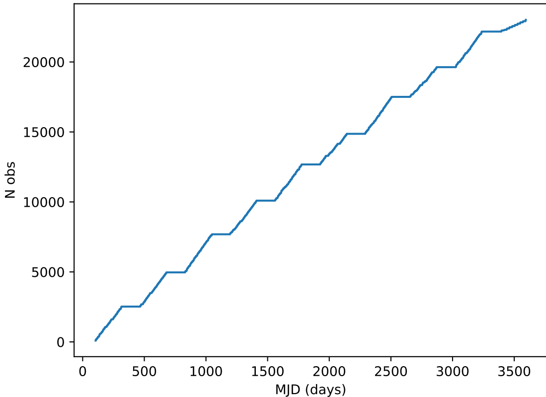
too_elab_r8_d2_giz_v3.4_10yrs all bands: DD:EDFS Cumulative NVisits
