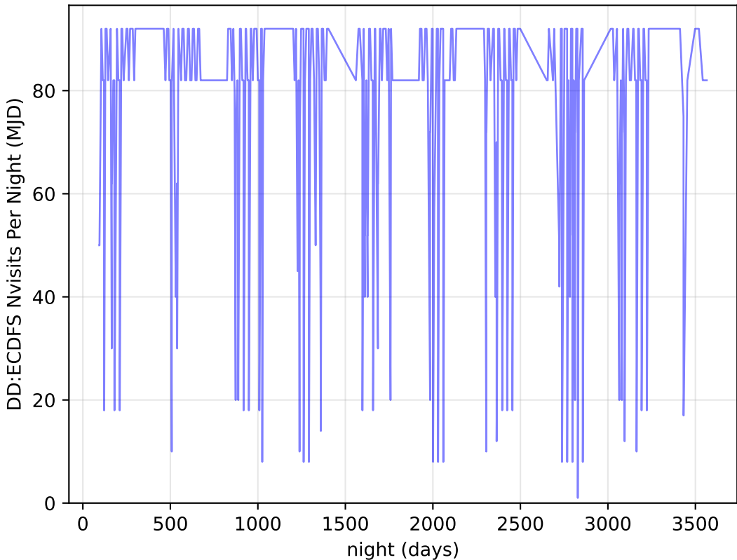
too_elab_r8_d2_giz_v3.4_10yrs all bands: DD:ECDFS Nvisits Per Night
