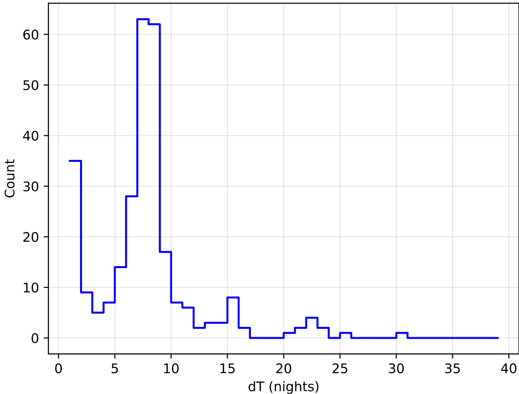
too_elab_r8_d2_giz_v3.4_10yrs all bands: DD:ECDFS Delta Nights Histogram
