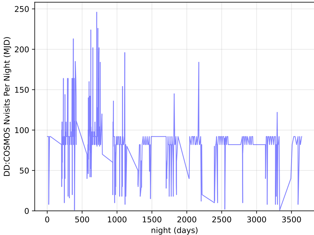
too_elab_r8_d2_giz_v3.4_10yrs all bands: DD: COSMOS Nvisits Per Night
