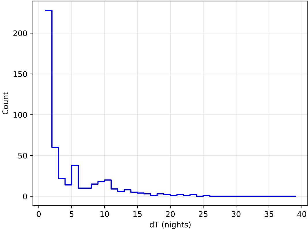
too_elab_r8_d2_giz_v3.4_10yrs all bands: DD: COSMOS Delta Nights Histogram
