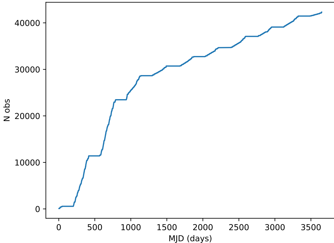
too_elab_r8_d2_giz_v3.4_10yrs all bands: DD: COSMOS Cumulative NVisits
