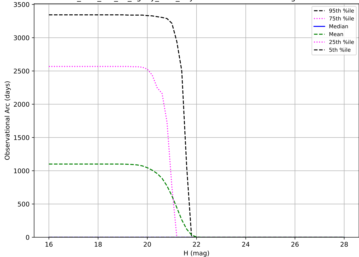
too_elab_r64_d3_ugrizy_v3.4_10yrs: Observational Arc Length Vatra
