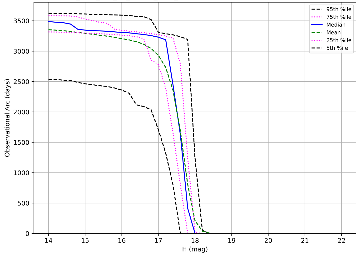
too_elab_r64_d3_ugrizy_v3.4_10yrs: Observational Arc Length Trojan
