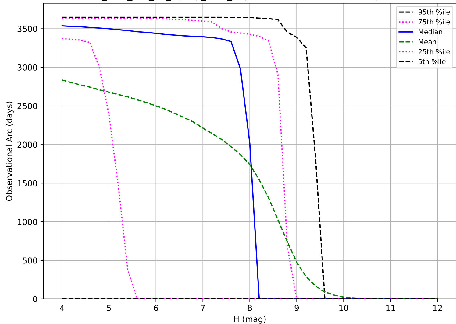
too_elab_r64_d3_ugrizy_v3.4_10yrs: Observational Arc Length TNO
