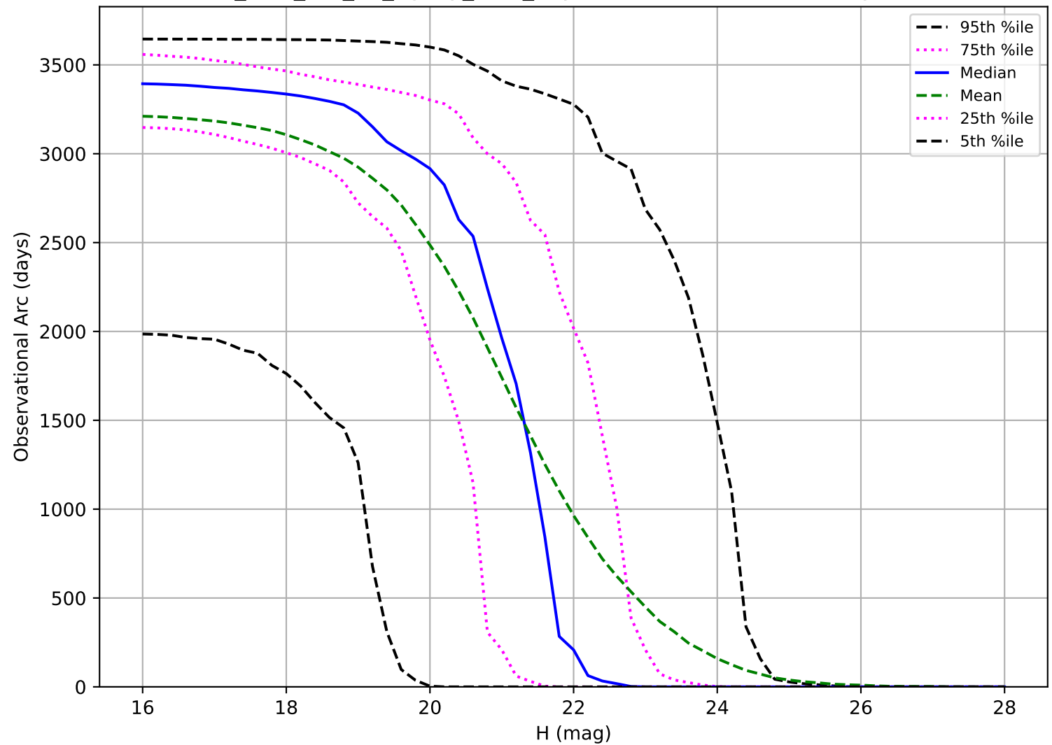
too_elab_r64_d3_ugrizy_v3.4_10yrs: Observational Arc Length PHA
