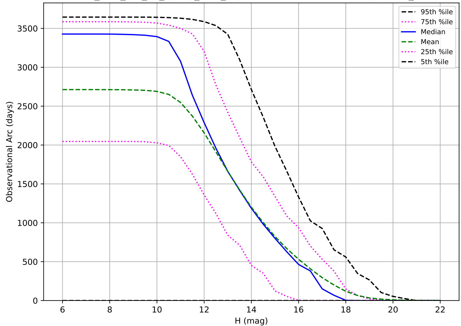
too_elab_r64_d3_ugrizy_v3.4_10yrs: Observational Arc Length OCC_r5
