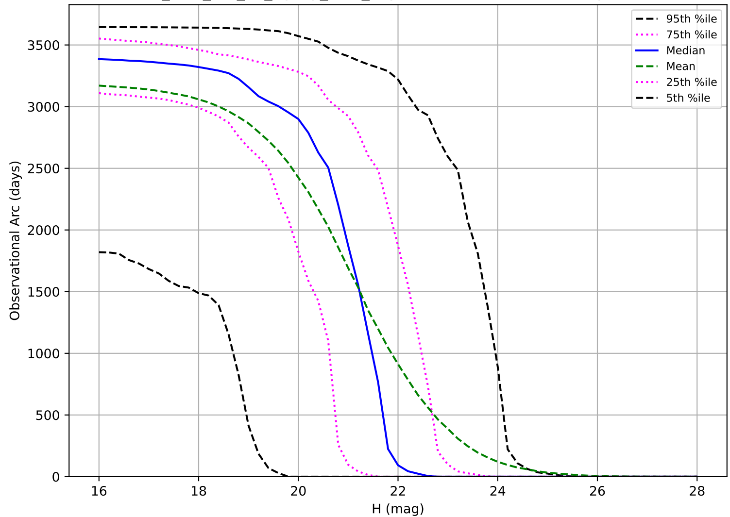
too_elab_r64_d3_ugrizy_v3.4_10yrs: Observational Arc Length NEO
