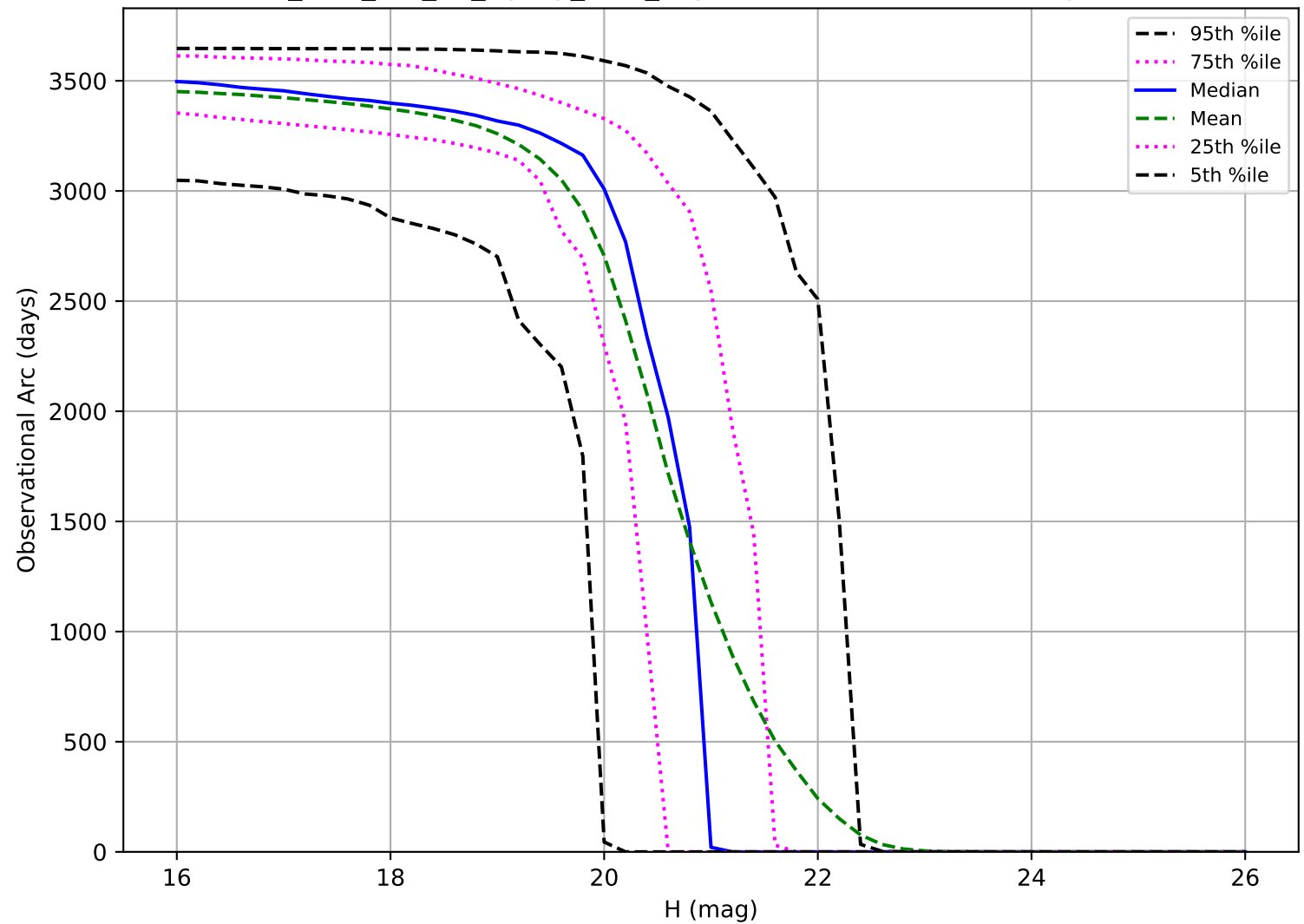
too_elab_r64_d3_ugrizy_v3.4_10yrs: Observational Arc Length MBA
