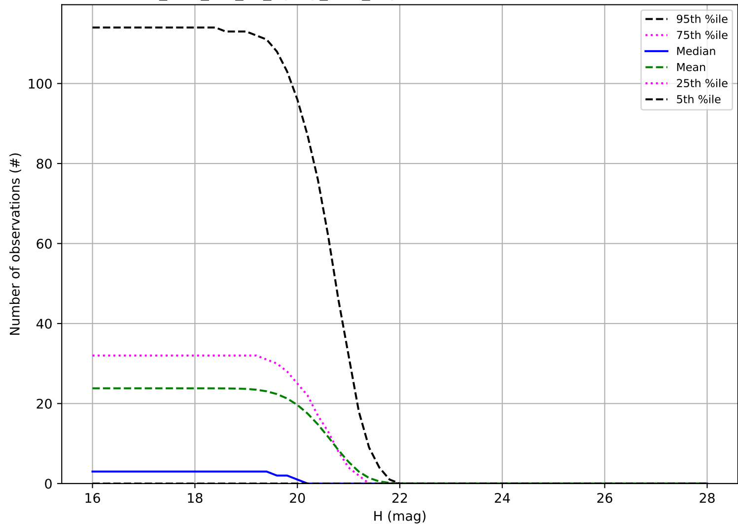
too_elab_r64_d3_ugrizy_v3.4_10yrs: Number of observations Vatira
