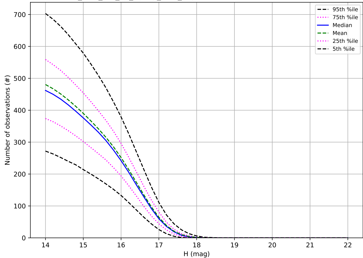
too_elab_r64_d3_ugrizy_v3.4_10yrs: Number of observations Trojan
