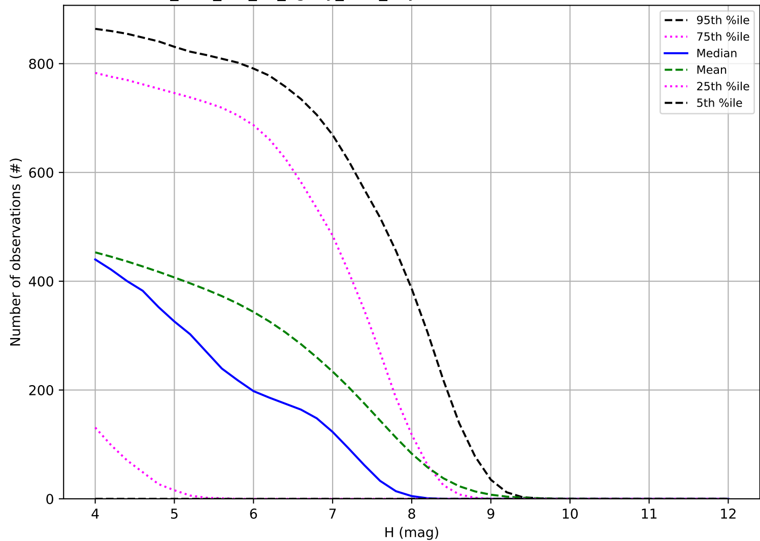
too_elab_r64_d3_ugrizy_v3.4_10yrs: Number of observations TNO
