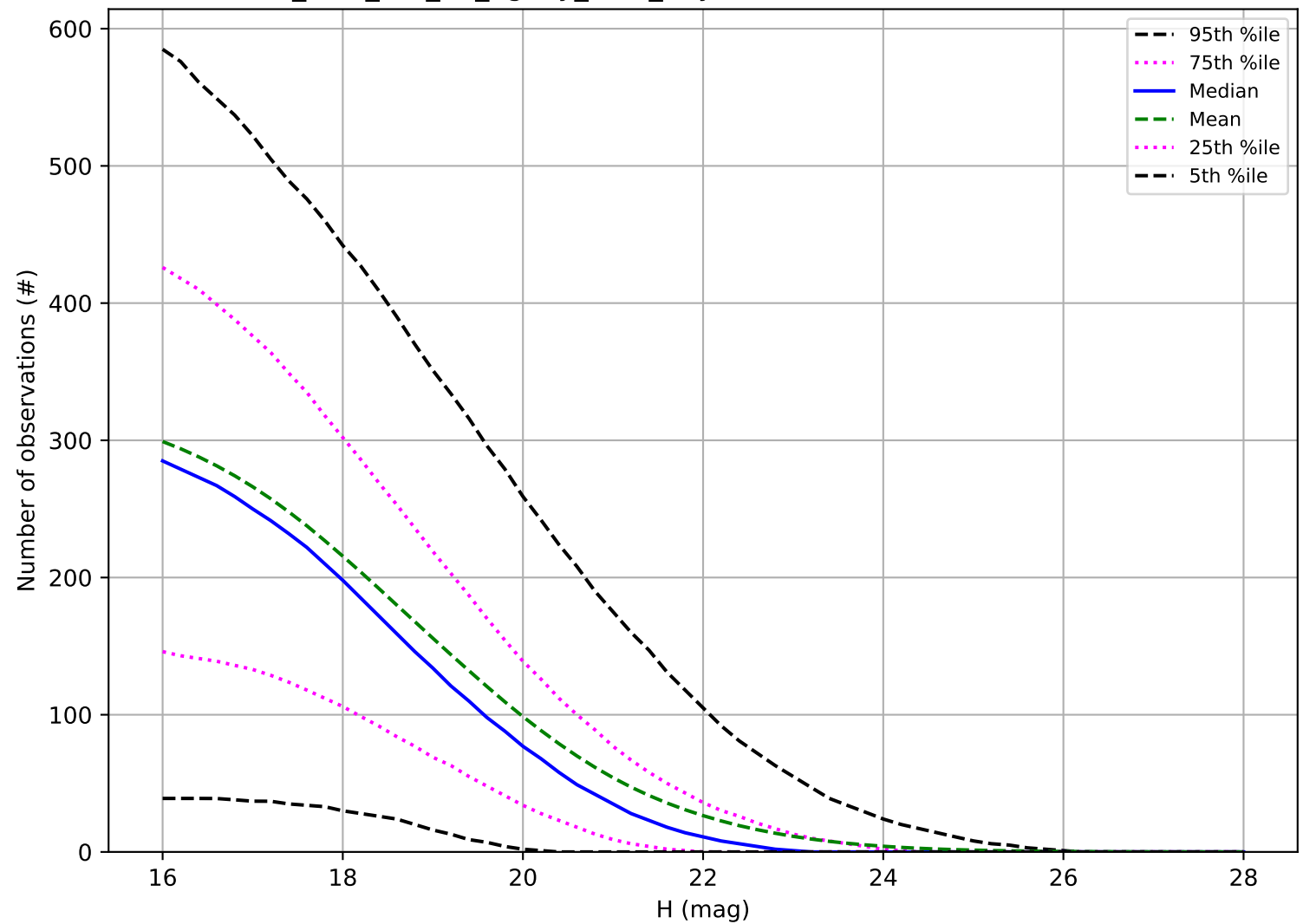
too_elab_r64_d3_ugrizy_v3.4_10yrs: Number of observations PHA
