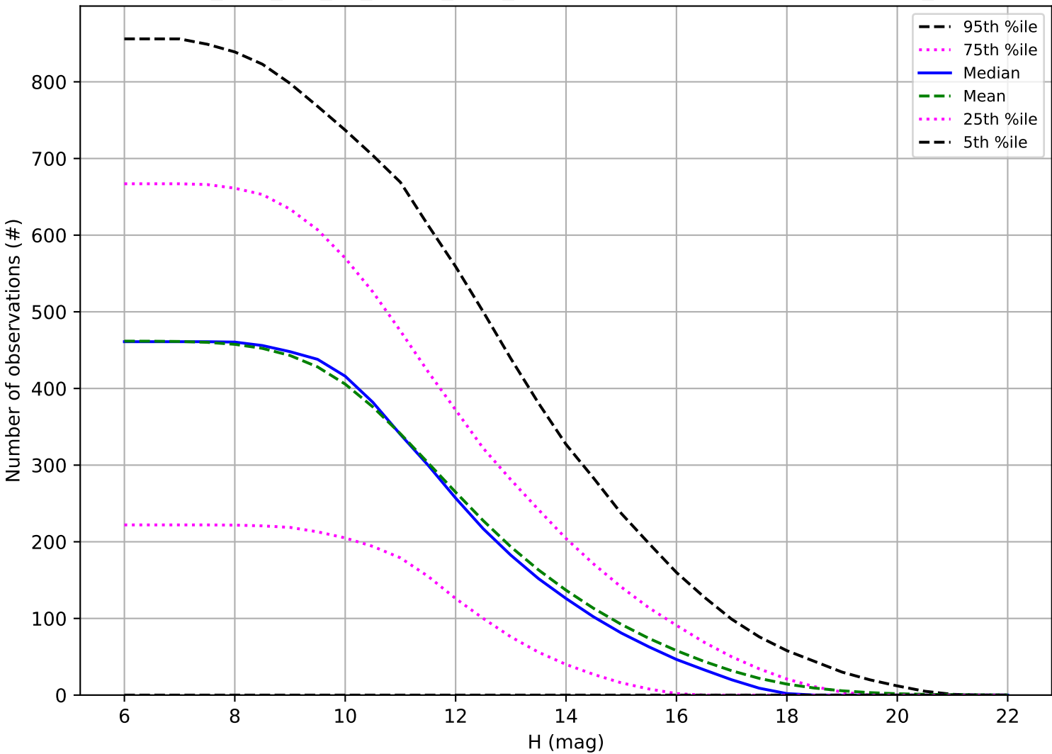
too_elab_r64_d3_ugrizy_v3.4_10yrs: Number of observations OCC_r5
