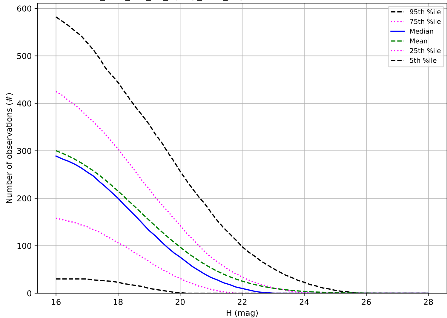
too_elab_r64_d3_ugrizy_v3.4_10yrs: Number of observations NEO
