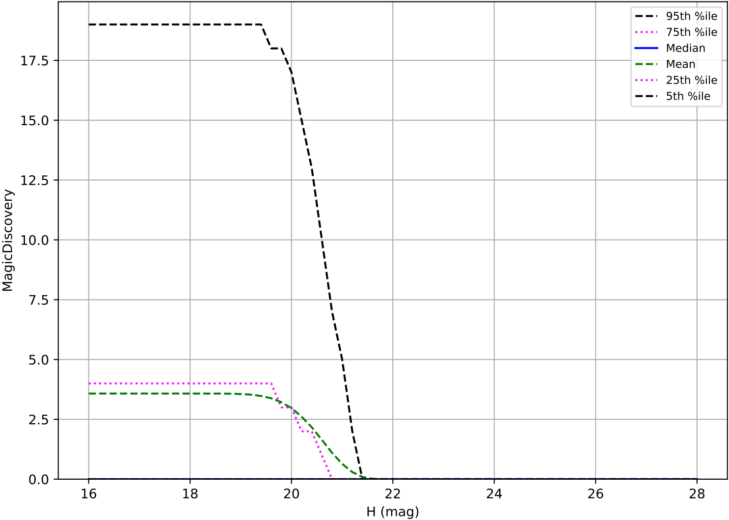
too_elab_r64_d3_ugrizy_v3.4_10yrs: Vatira 6 detections in 60 nights detection loss
