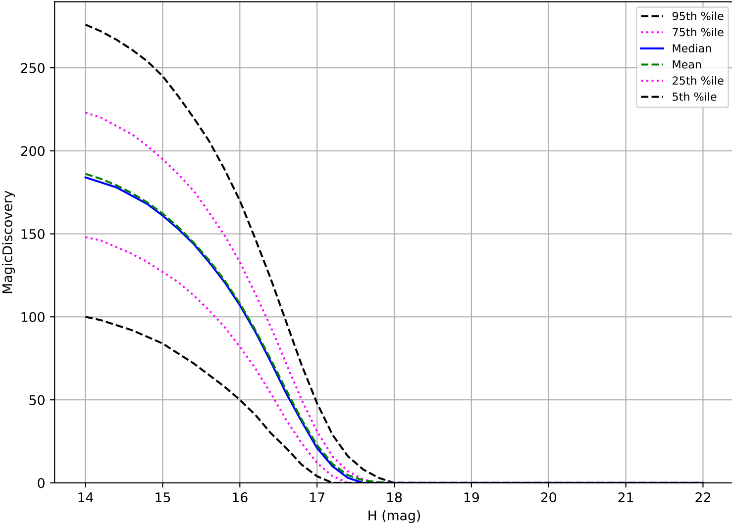
too_elab_r64_d3_ugrizy_v3.4_10yrs: Trojan 6 detections in 60 nights detection loss
