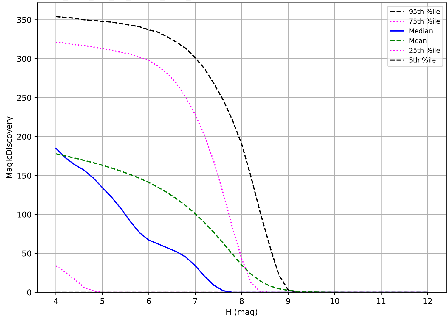
too_elab_r64_d3_ugrizy_v3.4_10yrs: TNO 6 detections in 60 nights detection loss
