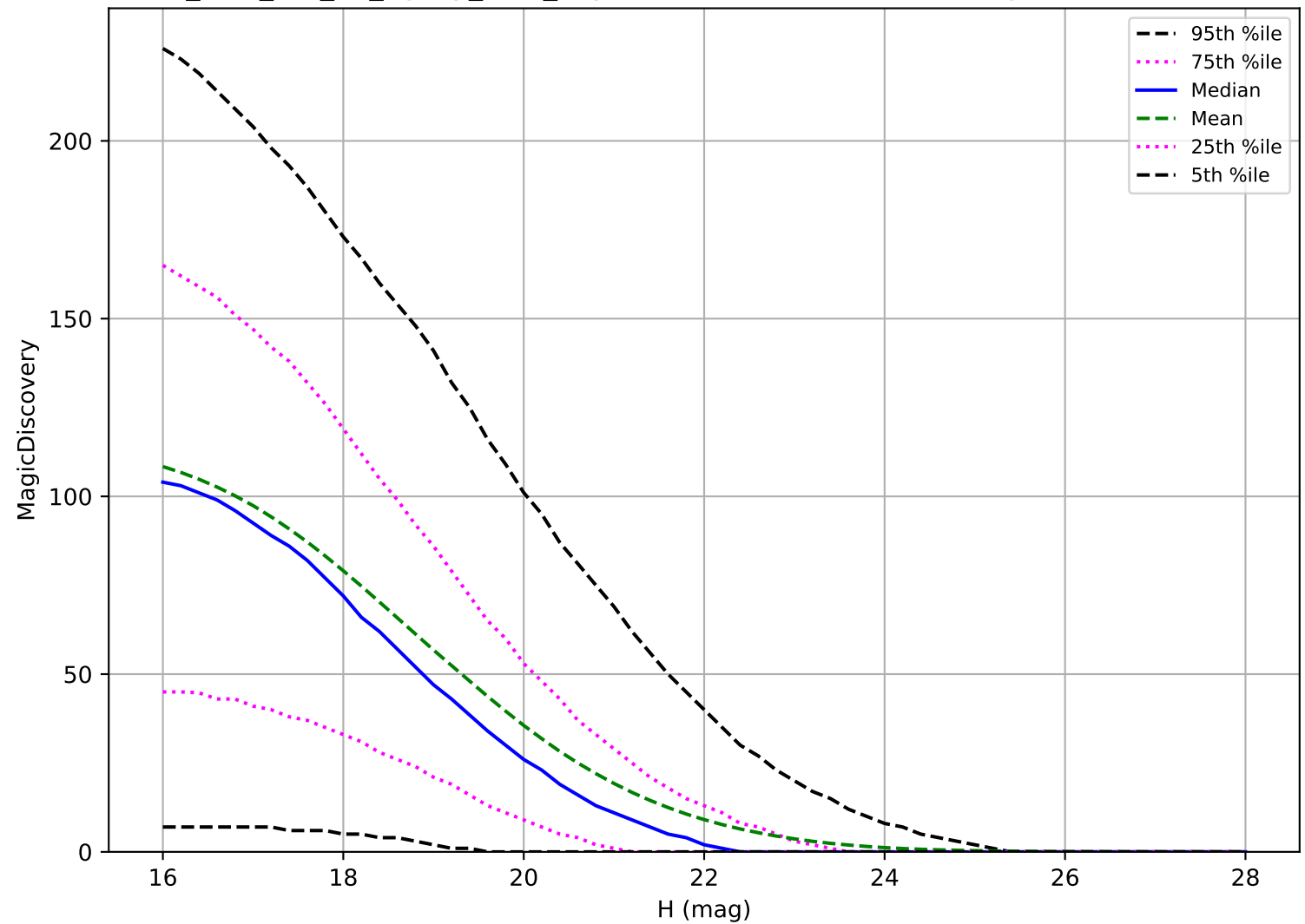
too_elab_r64_d3_ugrizy_v3.4_10yrs: PHA 6 detections in 60 nights detection loss
