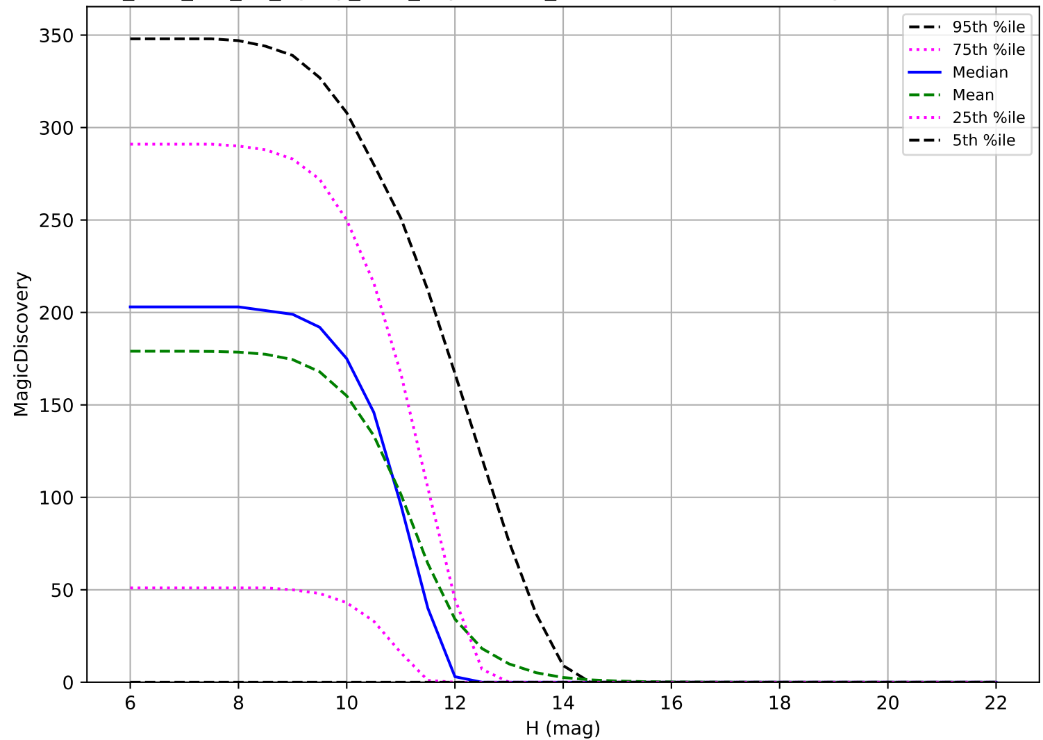
too_elab_r64_d3_ugrizy_v3.4_10yrs: OCC_r20 6 detections in 60 nights detection loss
