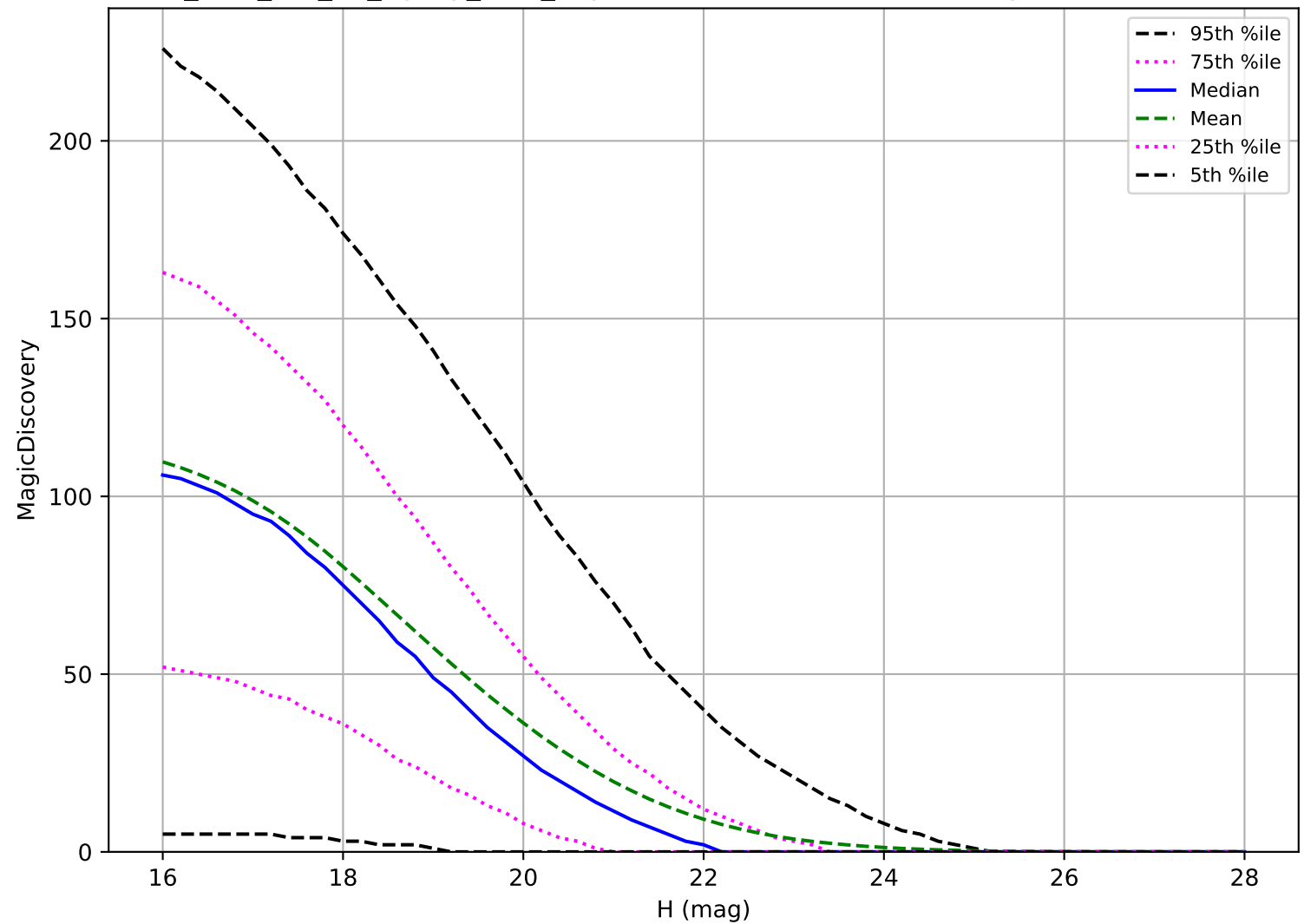
too_elab_r64_d3_ugrizy_v3.4_10yrs: NEO 6 detections in 60 nights detection loss
