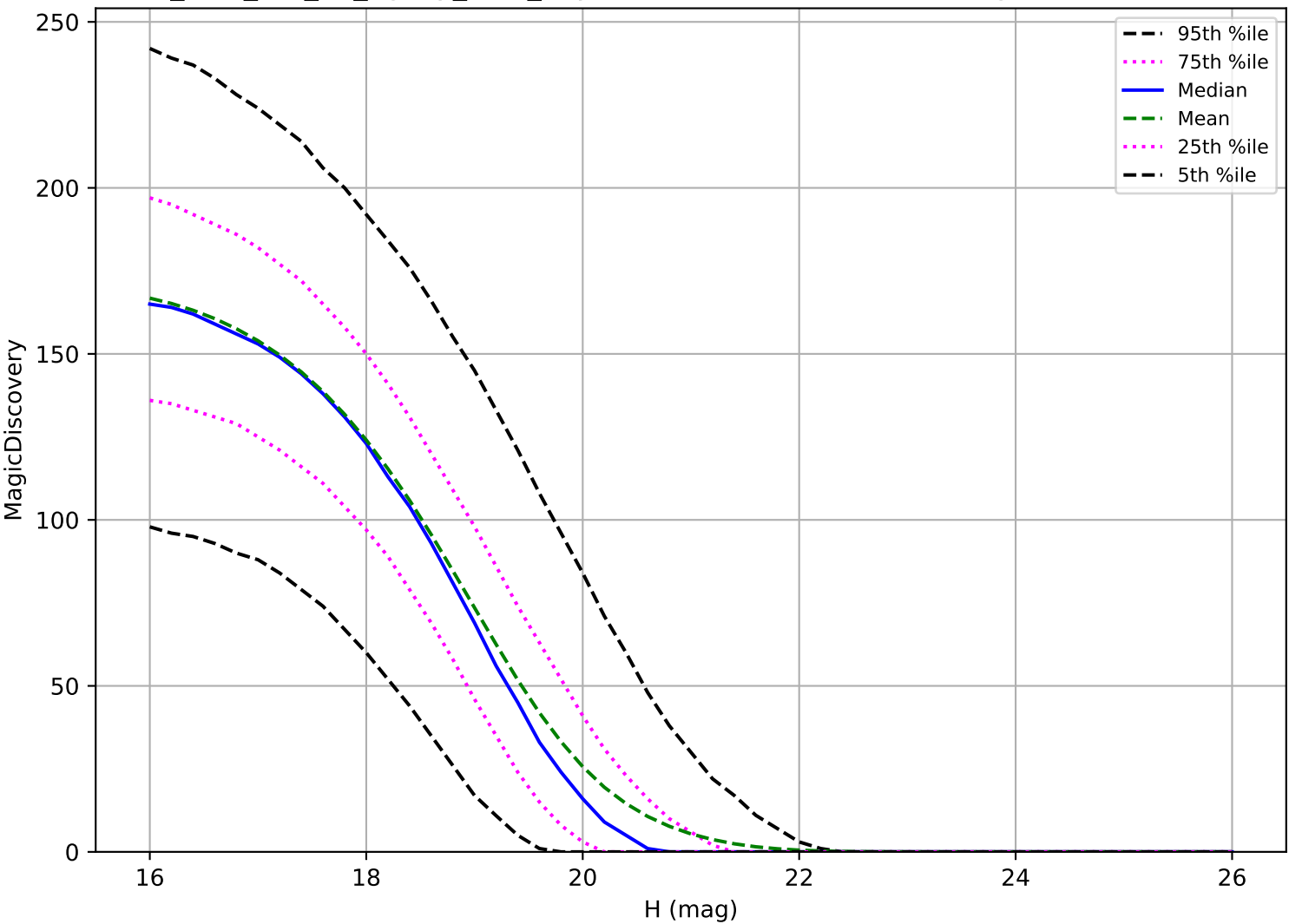
too_elab_r64_d3_ugrizy_v3.4_10yrs: MBA 6 detections in 60 nights detection loss
