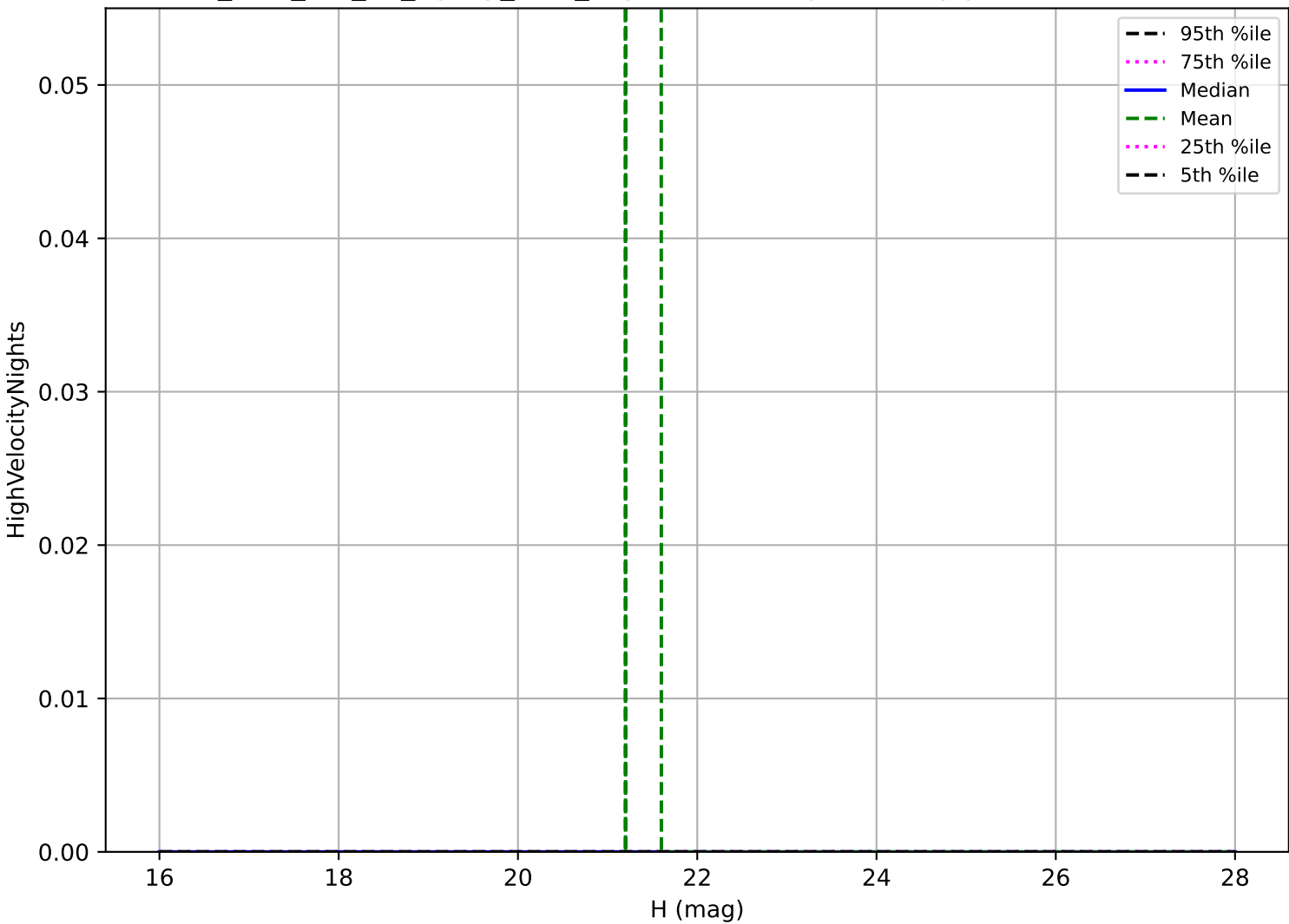
too_elab_r64_d3_ugrizy_v3.4_10yrs: Vatira High velocity pair detection loss
