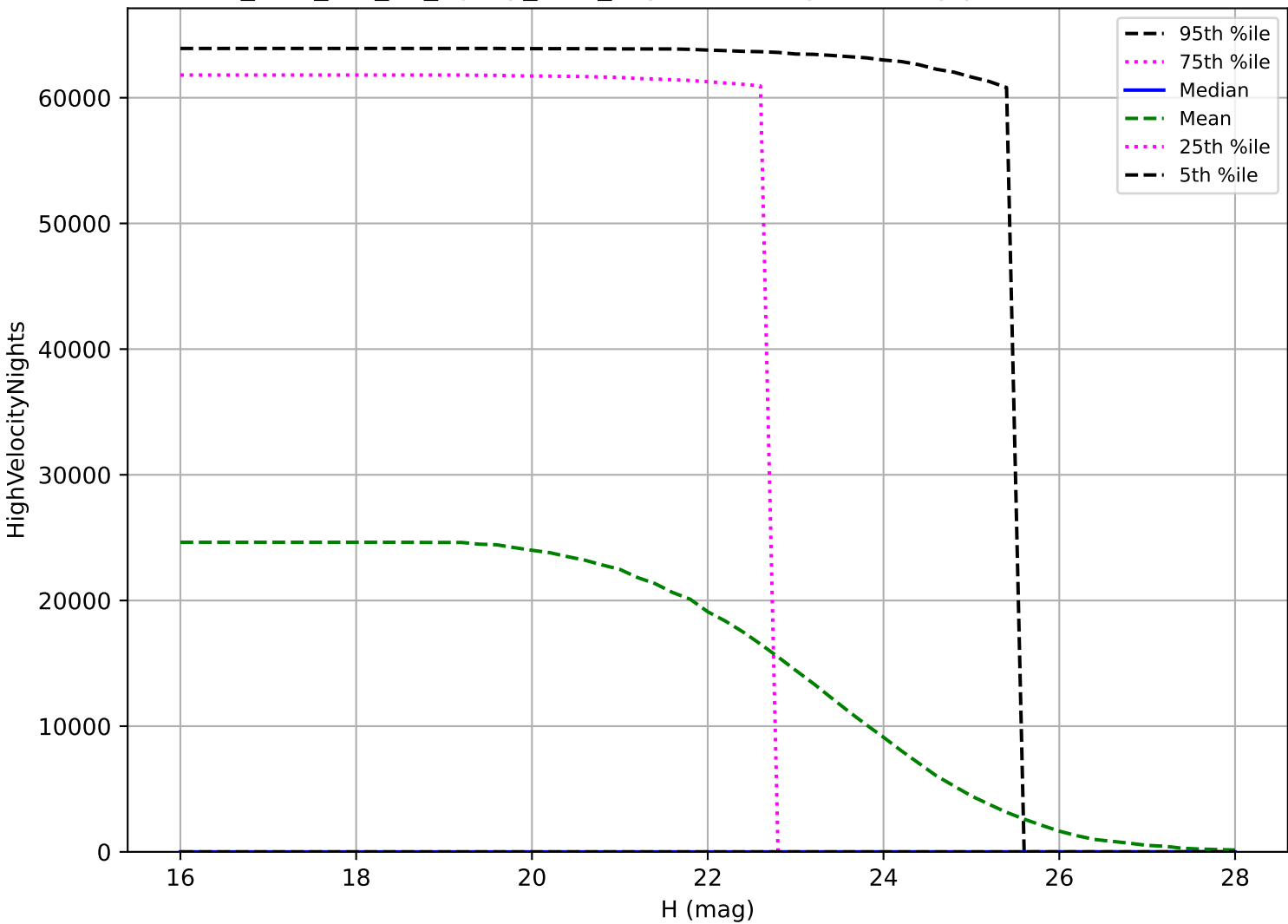
too_elab_r64_d3_ugrizy_v3.4_10yrs: PHA High velocity pair detection loss
