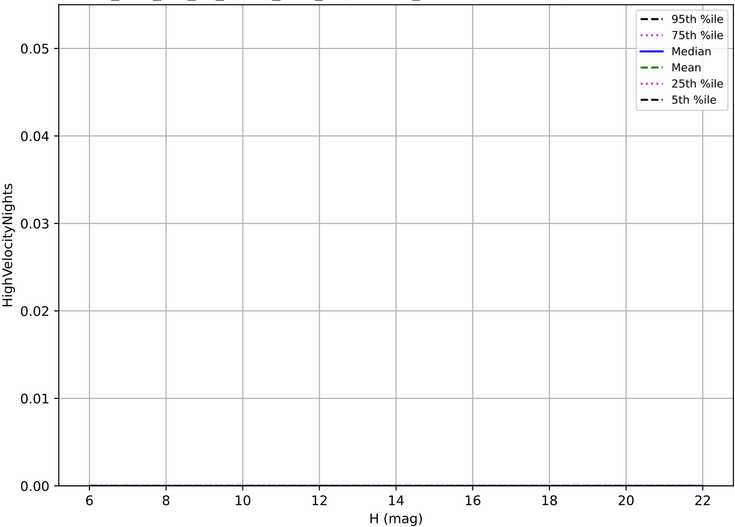
too_elab_r64_d3_ugrizy_v3.4_10yrs: OCC_r20 High velocity pair detection loss
