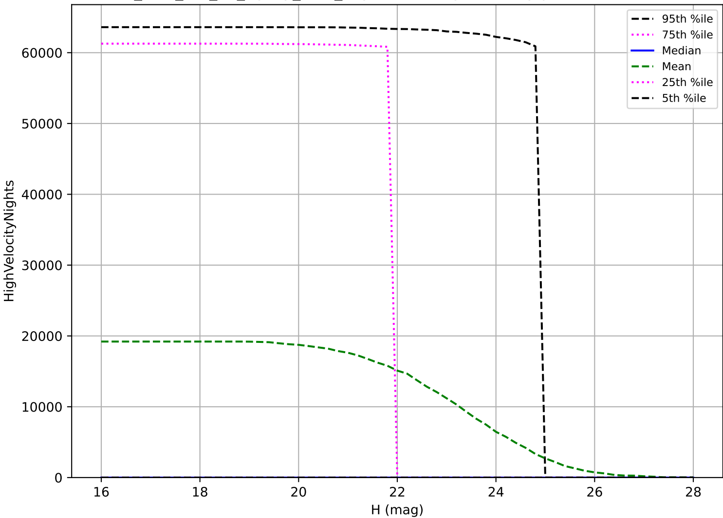
too_elab_r64_d3_ugrizy_v3.4_10yrs: NEO High velocity pair detection loss
