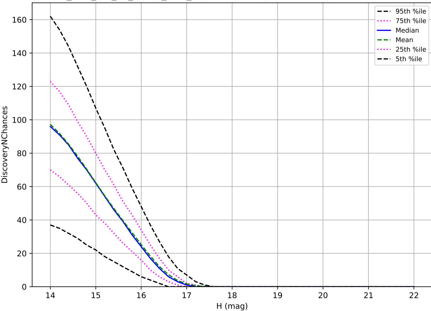
too_elab_r64_d3_ugrizy_v3.4_10yrs: Trojan 3 pairs in 15 nights detection loss
