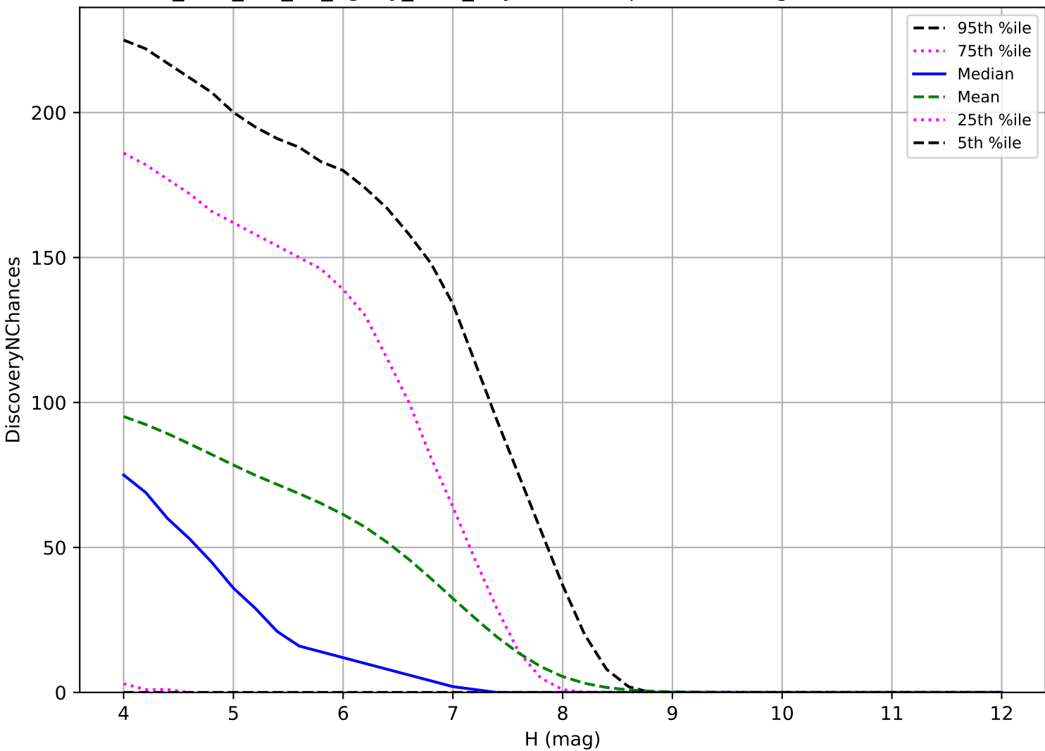
too_elab_r64_d3_ugrizy_v3.4_10yrs: TNO 3 pairs in 15 nights detection loss
