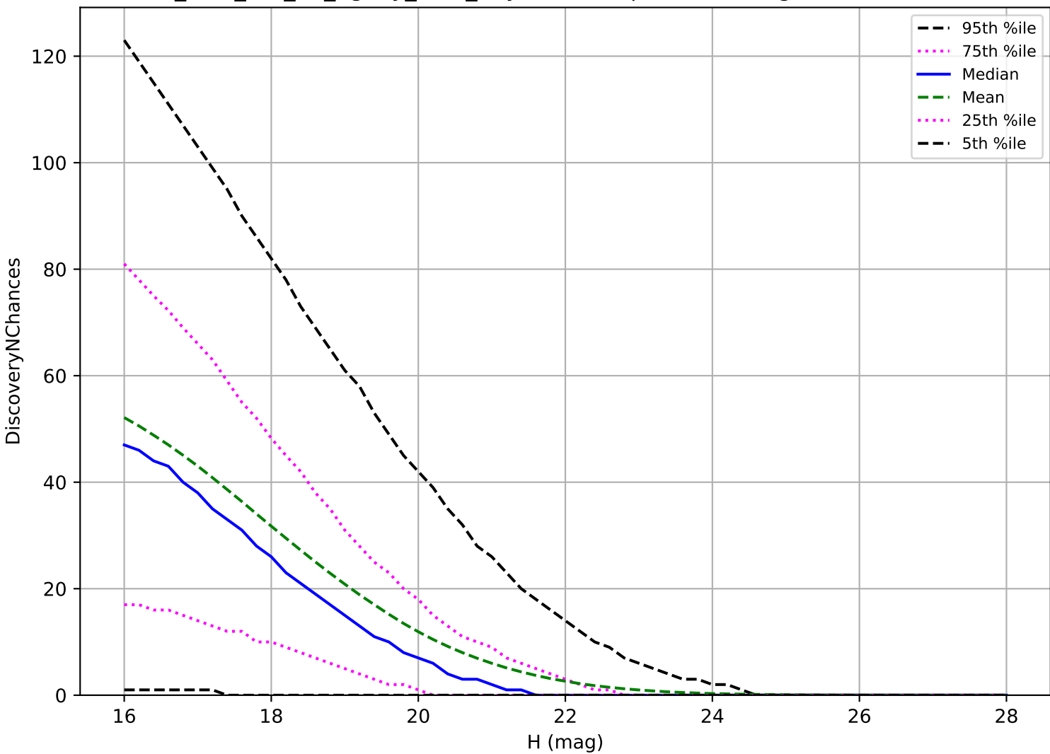
too_elab_r64_d3_ugrizy_v3.4_10yrs: PHA 3 pairs in 15 nights detection loss
