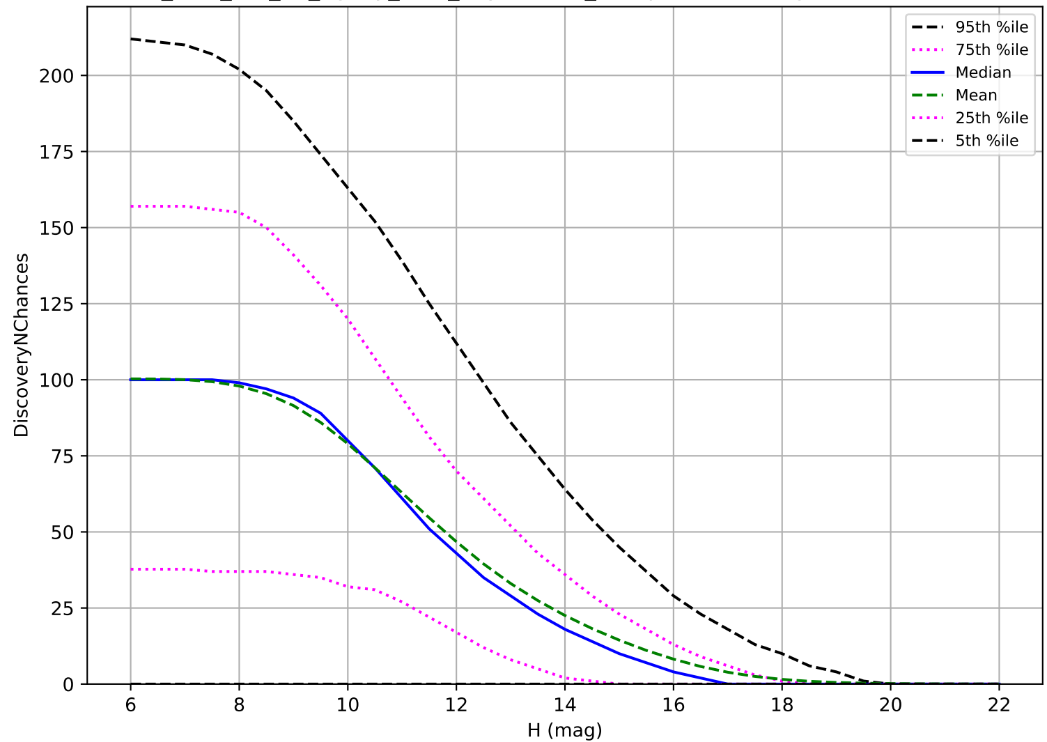
too_elab_r64_d3_ugrizy_v3.4_10yrs: OCC_r5 3 pairs in 15 nights detection loss
