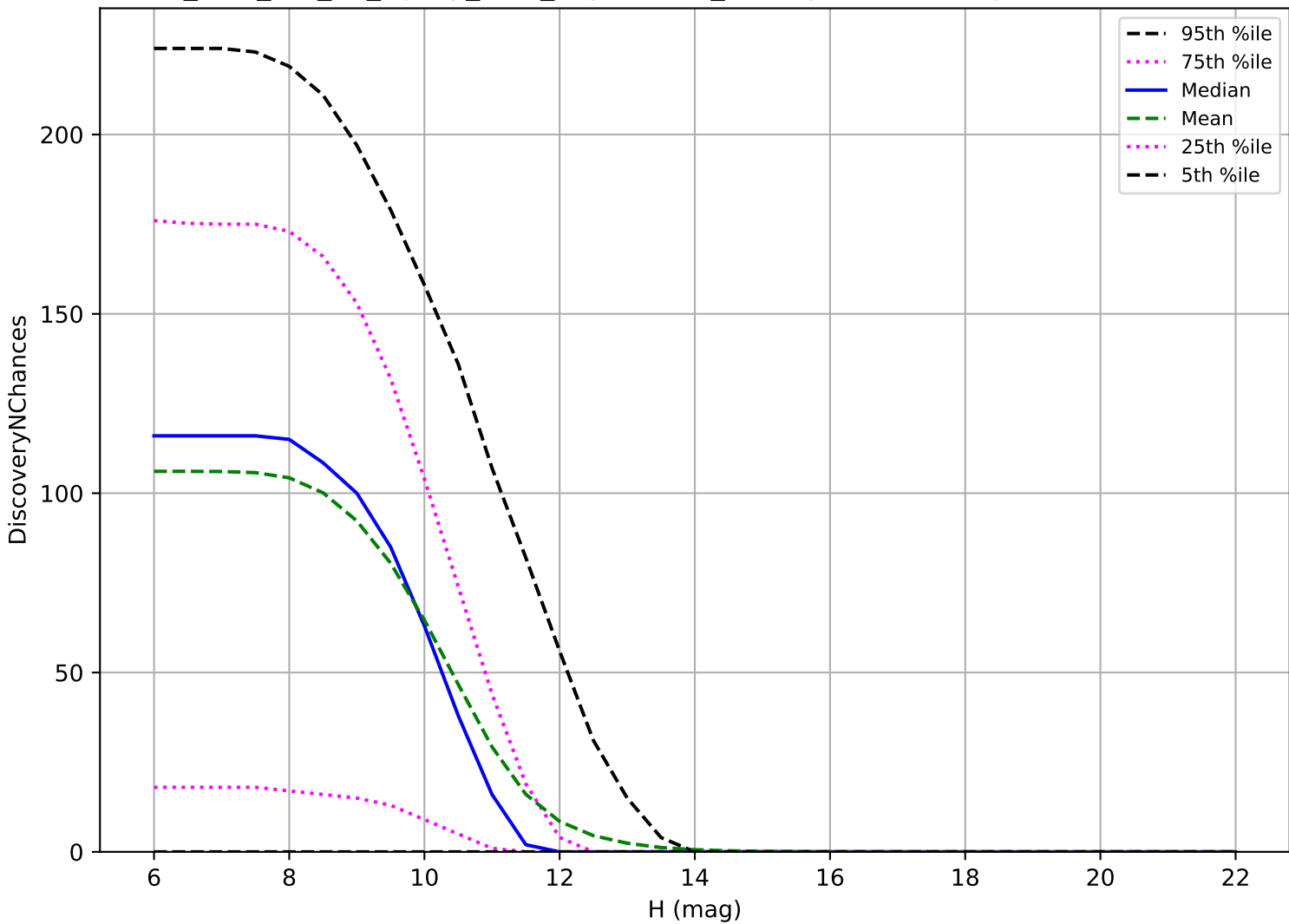
too_elab_r64_d3_ugrizy_v3.4_10yrs: OCC_r20 3 pairs in 15 nights detection loss
