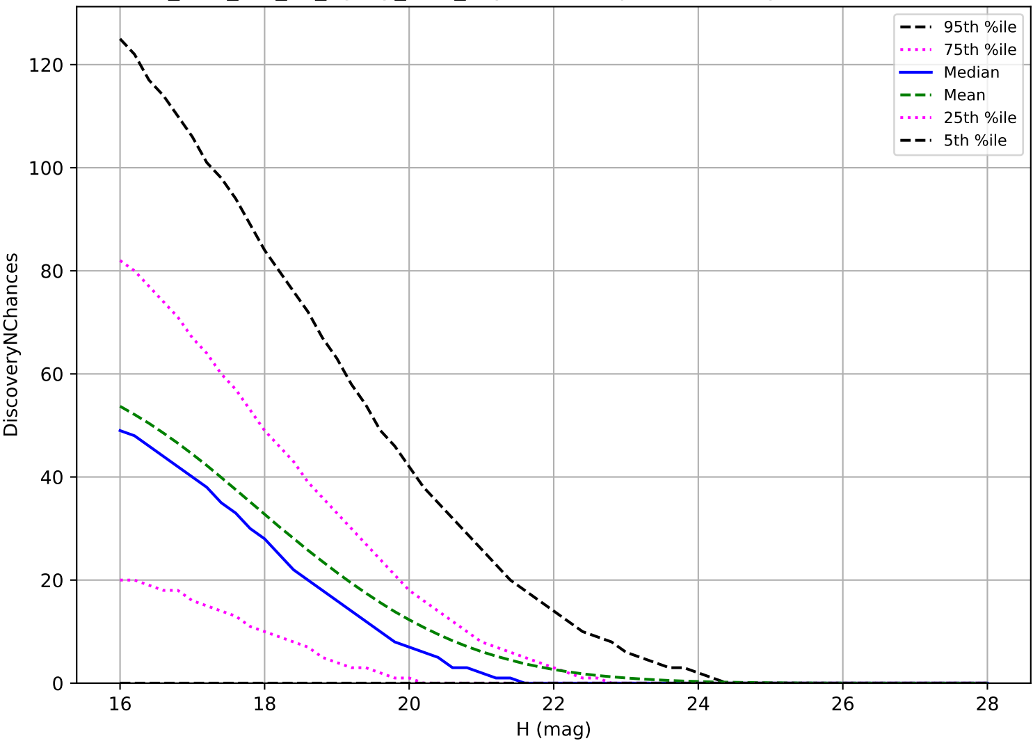
too_elab_r64_d3_ugrizy_v3.4_10yrs: NEO 3 pairs in 15 nights detection loss
