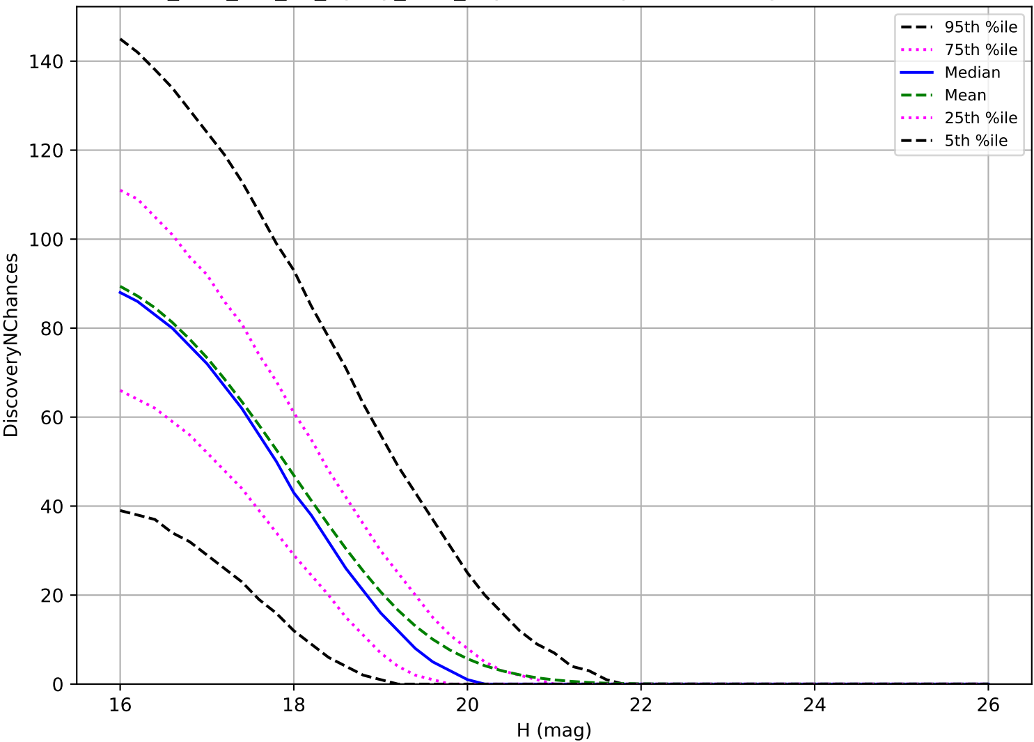
too_elab_r64_d3_ugrizy_v3.4_10yrs: MBA 3 pairs in 15 nights detection loss
