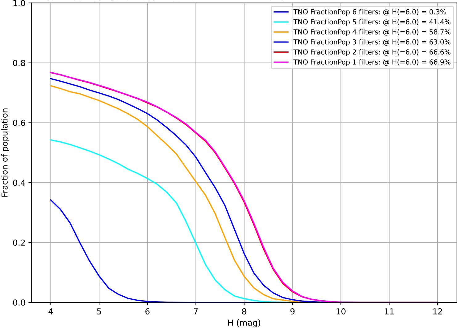
too_elab_r64_d3_ugrizy_v3.4_10yrs: Fraction of population with colors in X filters TNO
