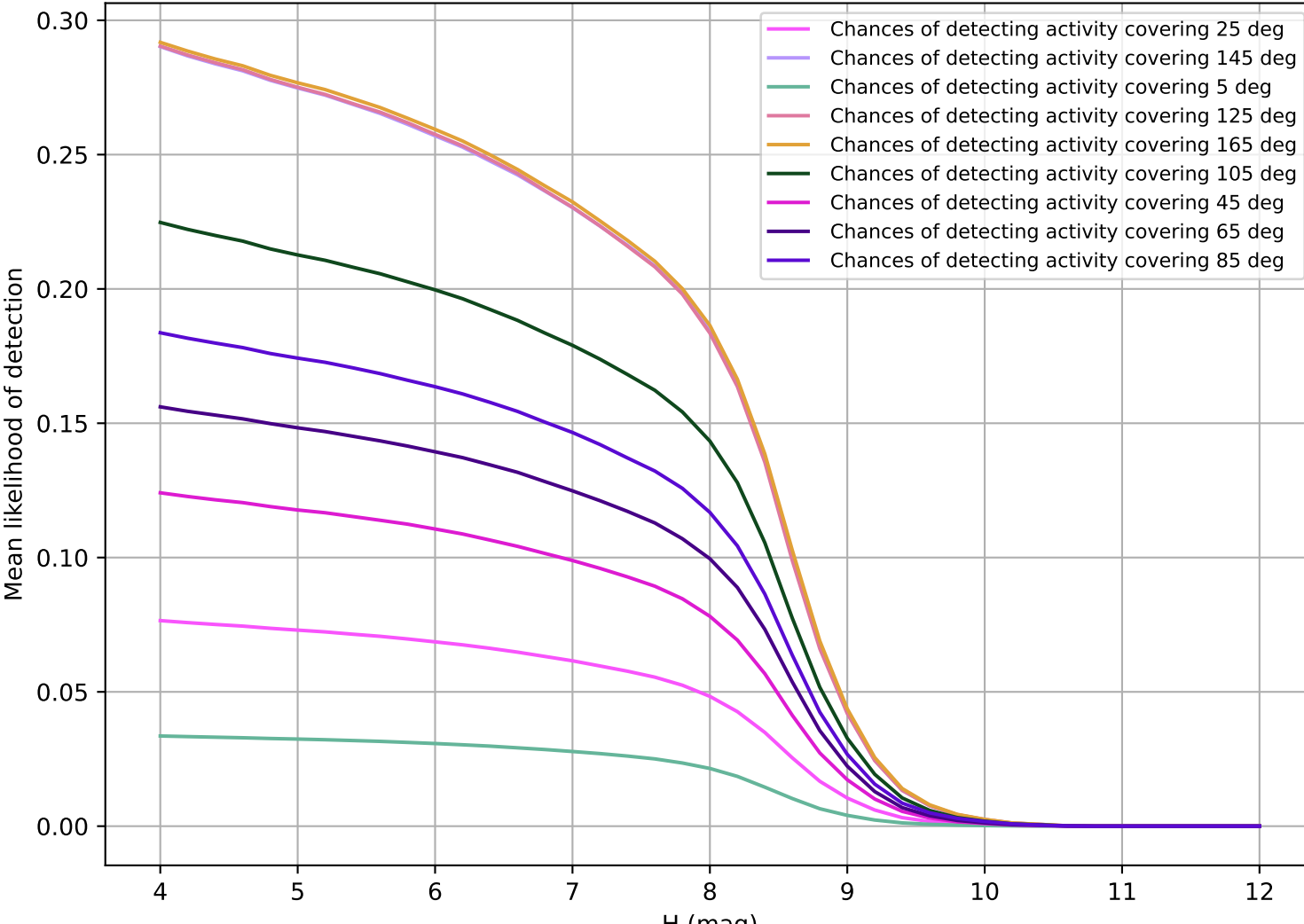
too_elab_r64_d3_ugrizy_v3.4_10yrs TNO
