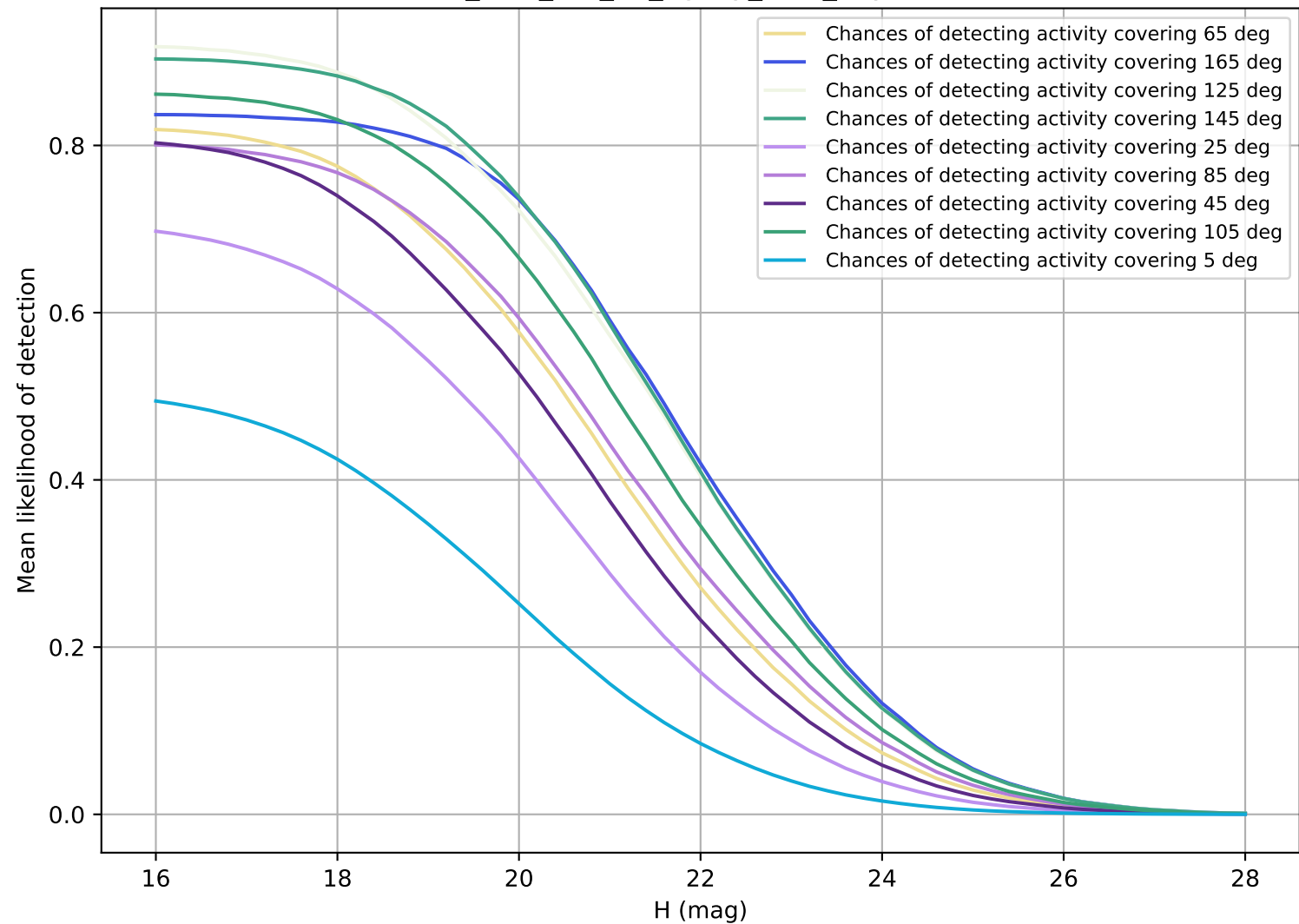
too_elab_r64_d3_ugrizy_v3.4_10yrs PHA
