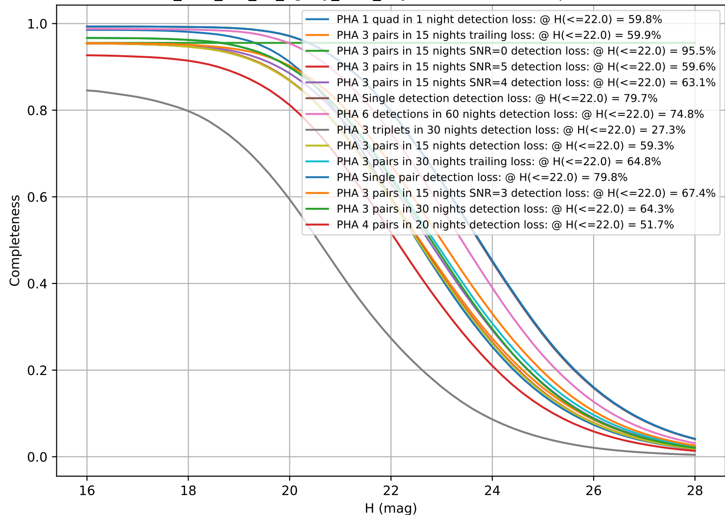
too_elab_r64_d3_ugrizy_v3.4_10yrs: CumulativeCompleteness
