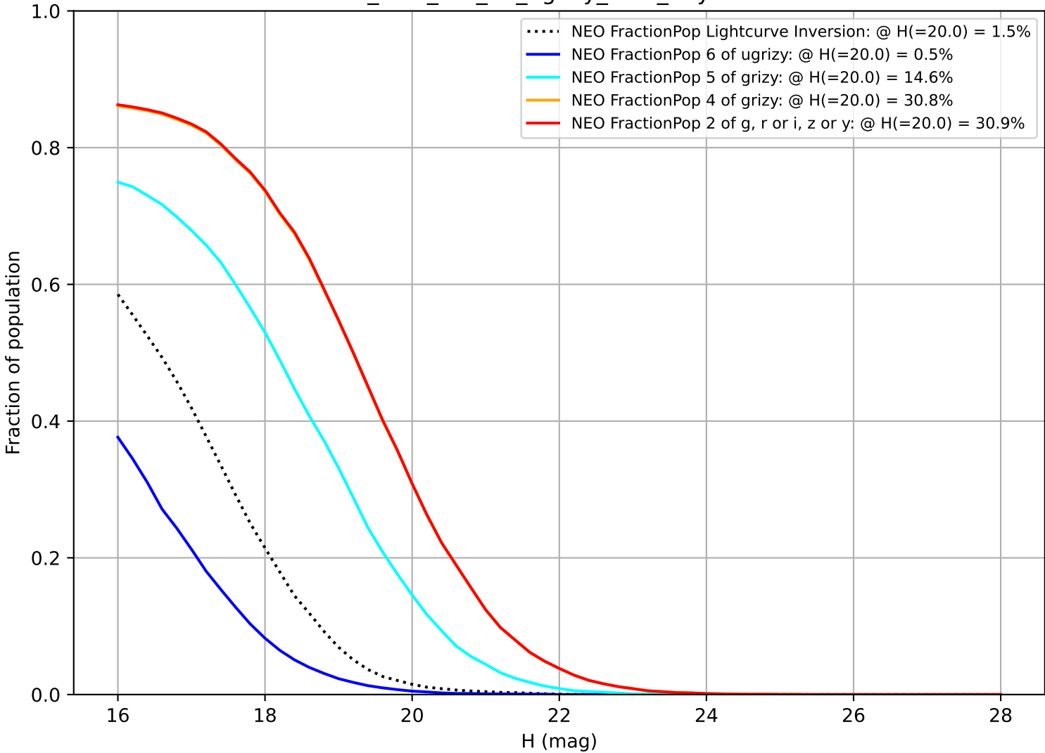
too_elab_r64_d3_ugrizy_v3.4_10yrs NEO
