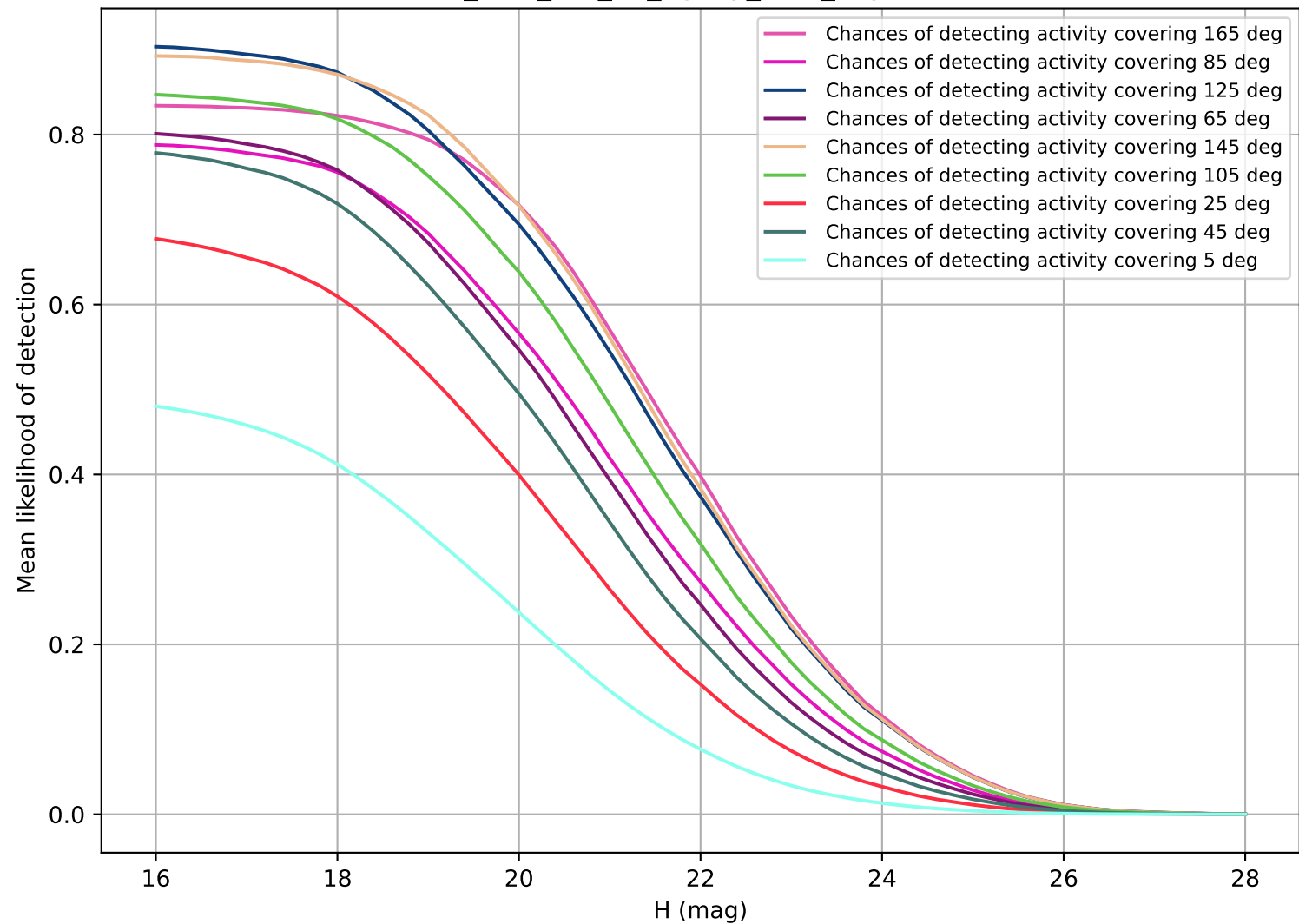
too_elab_r64_d3_ugrizy_v3.4_10yrs NEO
