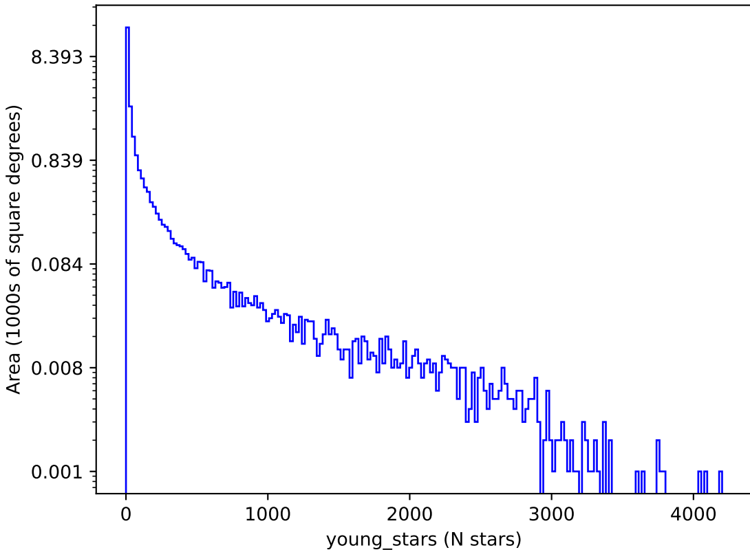
too_elab_r64_d3_ugrizy_v3.4_10yrs : young_stars
