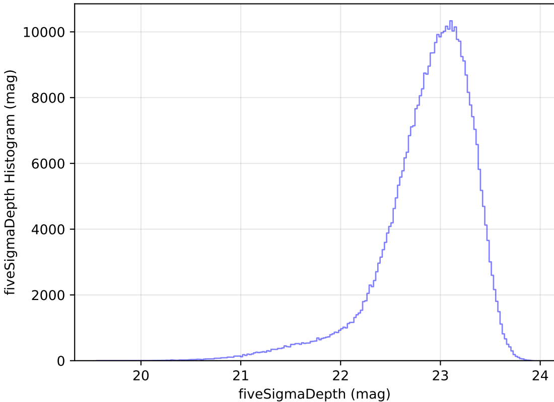
too_elab_r64_d3_ugrizy_v3.4_10yrs z: fiveSigmaDepth Histogram
